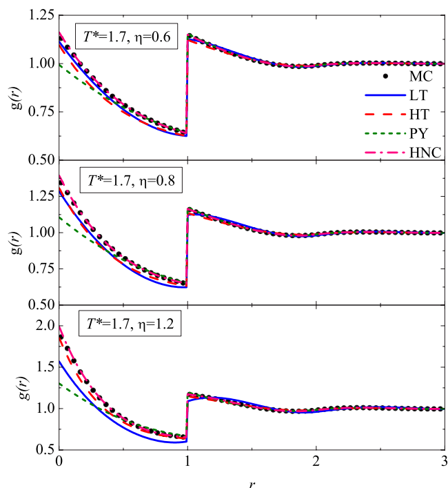
FIG. 6. (Color online) Plot of the radial distribution function at T^*=1.7 and for densities \eta=0.6 , \eta=0.8 , and \eta=1.2 . The circles are MC simulation data, while the lines correspond to the LT approximation (—), the HT approximation (---), the PY theory (- - -), and the HNC theory (-·-).
