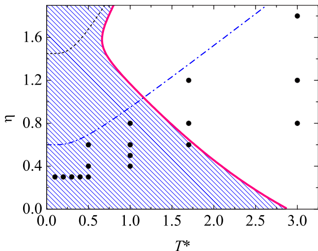
FIG. 8. (Color online) The circles represent the states considered in Figs. 3–7. The thick solid line represents the locus of points where the LT and HT approximations predict the same value of the contact quantity y(1)=g(1^+) . The LT approximation is more accurate in the shaded region to the left of the curve, while the HT approximation is more accurate to the right of the curve. The dashed-dotted line is a rough estimate of the freezing curve, while the dashed line represents the threshold curve (Kirkwood’s instability line) above which the HT theory ceases to exist.
