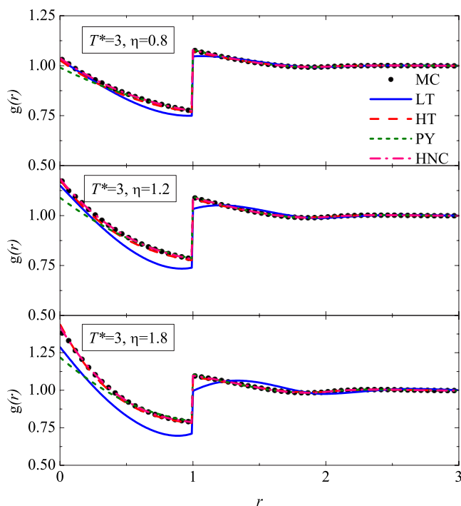
FIG. 7. (Color online) Plot of the radial distribution function at T^*=3 and for densities \eta=0.8 , \eta=1.2 , and \eta=1.8 . The circles are MC simulation data, while the lines correspond to the LT approximation (—), the HT approximation (---), the PY theory (···), and the HNC theory (-·-·).
