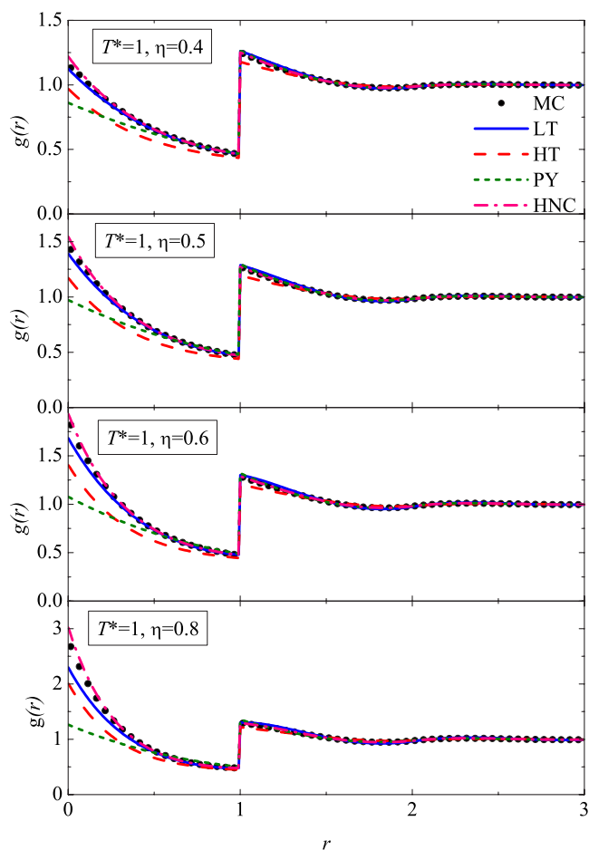
FIG. 5. (Color online) Plot of the radial distribution function at T^*=1 and for densities \eta=0.4 , \eta=0.5 , \eta=0.6 , and \eta=0.8 . The circles are MC simulation data, while the lines correspond to the LT approximation (—), the HT approximation (---), the PY theory (- - -), and the HNC theory (-·-).
