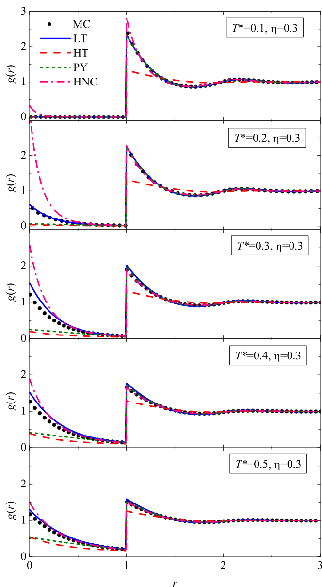
FIG. 3. (Color online) Plot of the radial distribution function at \eta=0.3 and for temperatures T^*=0.1 , T^*=0.2 , T^*=0.3 , T^*=0.4 , and T^*=0.5 . The circles are MC simulation data, while the lines correspond to the LT approximation (—), the HT approximation (---), the PY theory (· · ·), and the HNC theory (-·-·).
