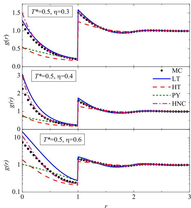
FIG. 4. (Color online) Plot of the radial distribution function at T^*=0.5 and for densities \eta=0.3 , \eta=0.4 , and \eta=0.6 . The circles are MC simulation data, while the lines correspond to the LT approximation (—), the HT approximation (---), the PY theory (· · ·), and the HNC theory (-·-·).
